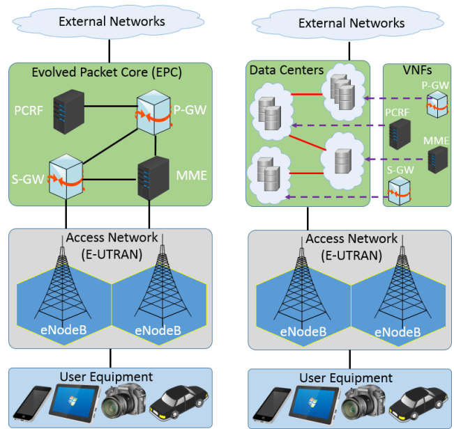
Fig. 3. Virtualization of the EPC
